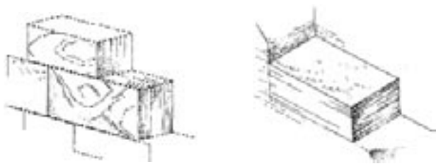
Brownstone can be laid with its natural bedding planes oriented vertically, called face bedding (left), or horizontally, called quarry bedding (right).
